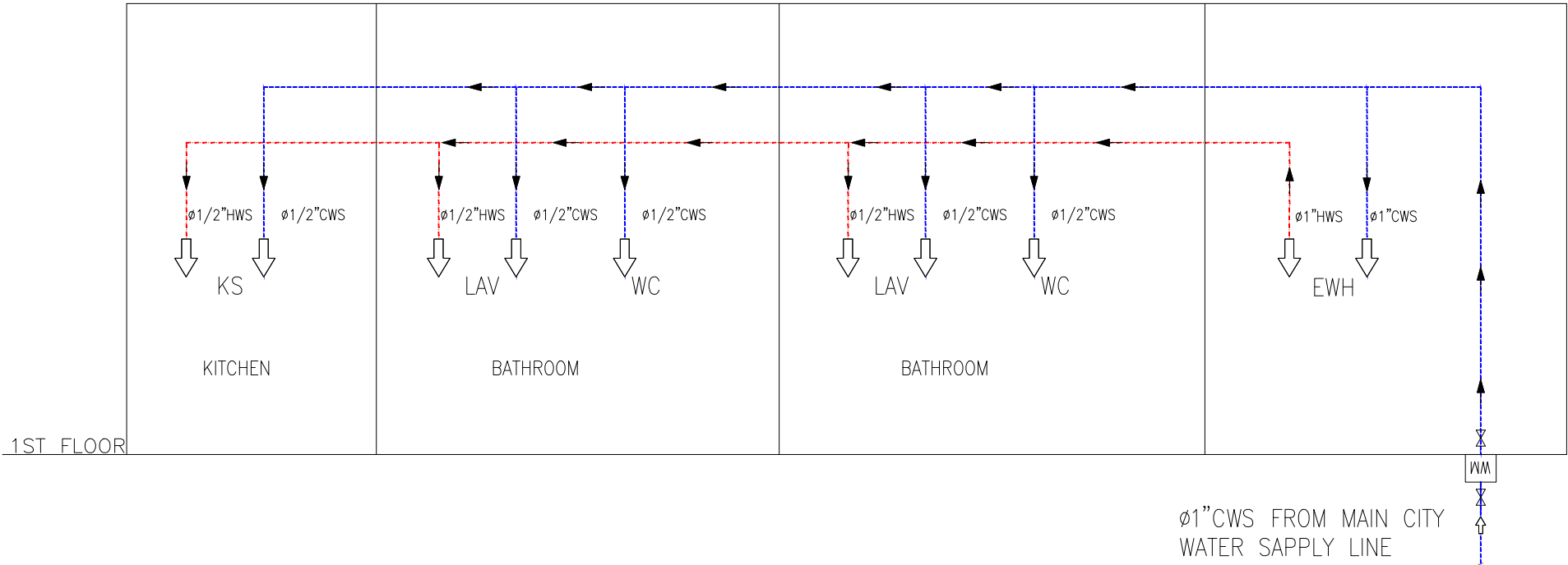
PL 03 WATER SUPPLY SYSTEM RISER DIAGRAM SCALE NTS
