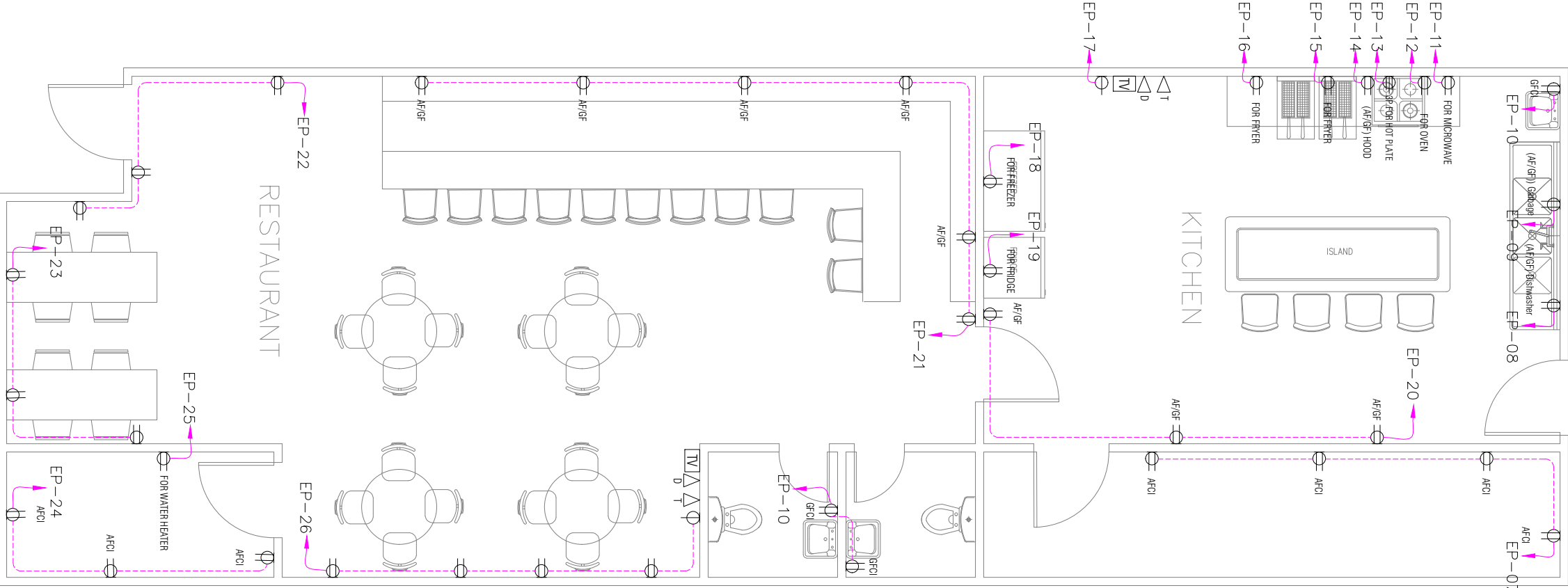
EL 02 POWER FLOOR PLAN SCALE 3/16"=1'-0"
