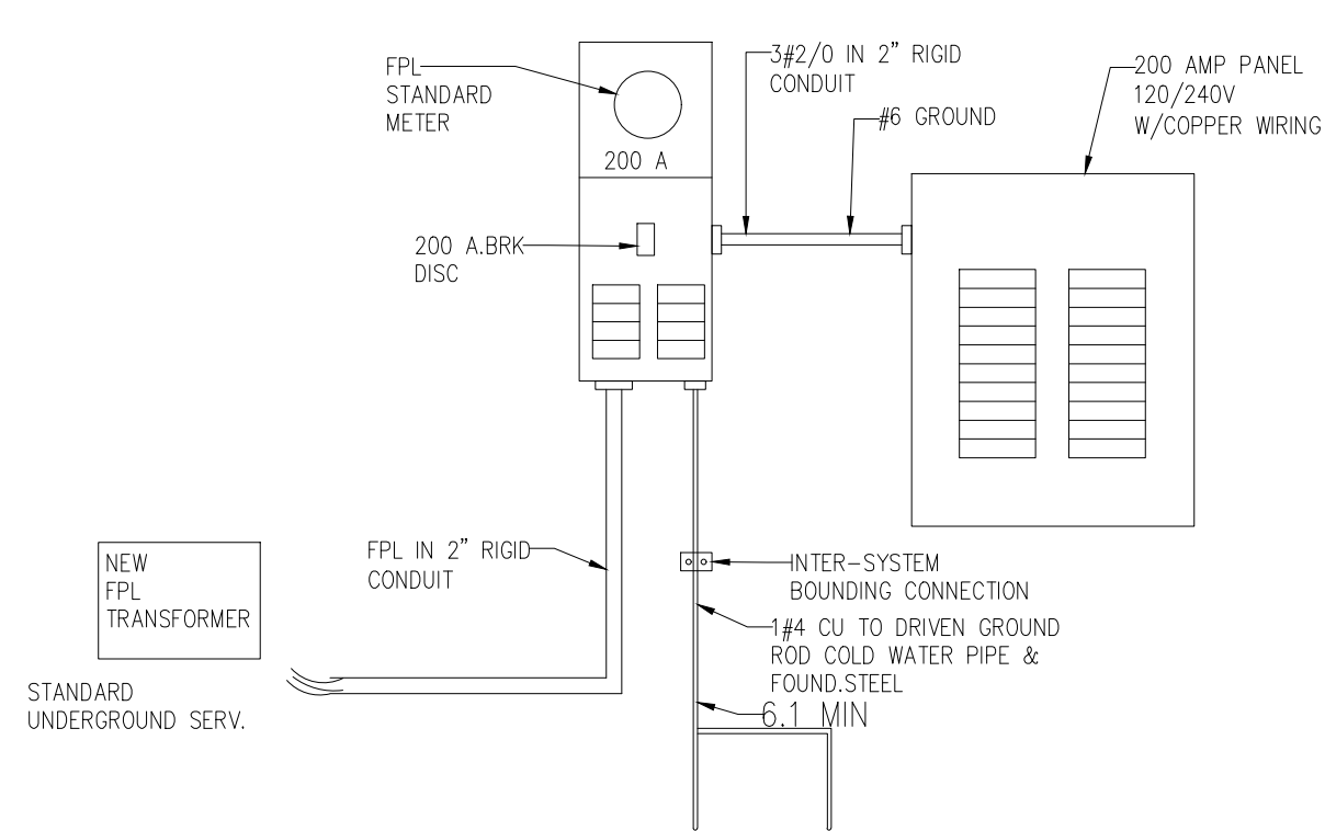
EL 03 SINGLE LINE DIAGRAM SCALE NTS
