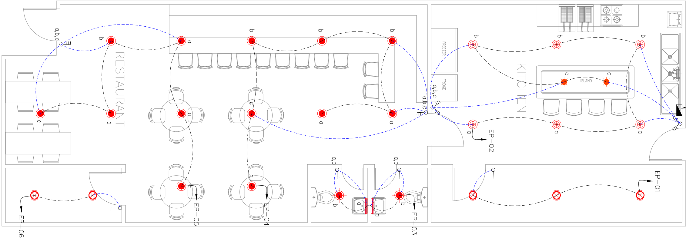
EL 02 LIGHTING FLOOR PLAN SCALE 3/16"=1'-0"
